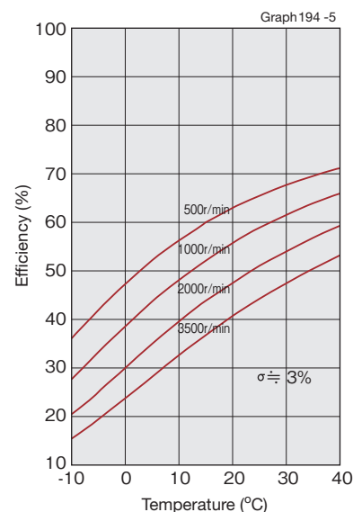
SHG/SHF-14 to 65 Reduction ratio 160
