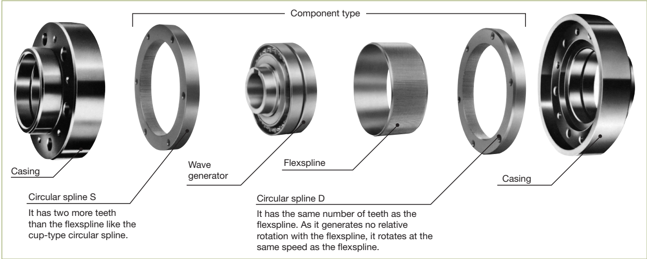
Structure of the FD series
