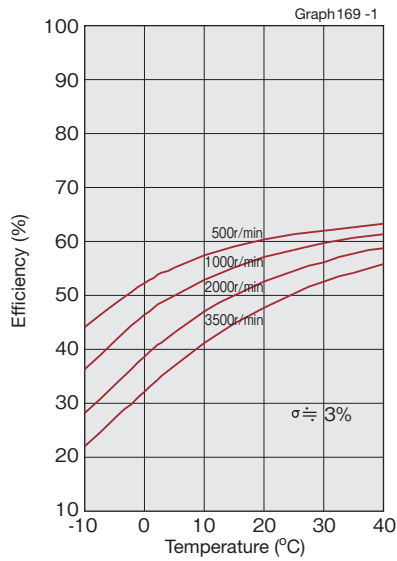
Model 14/ Reduction ratio 50
