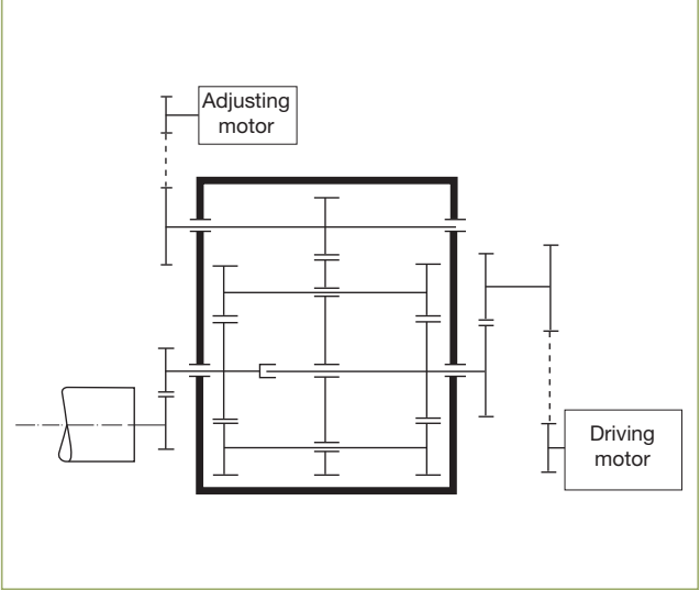
Conventional differential gear
