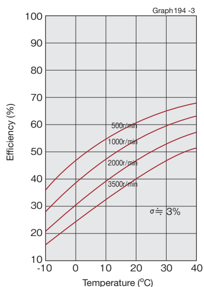
SHG/SHF-14 to 65 Reduction ratio 30
