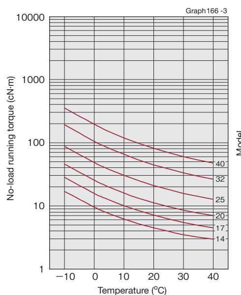
Input rotational speed: 2000r/min
