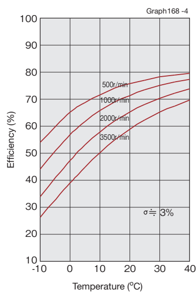
Model 17 to 50/ Reduction ratio 80, 100, 120
