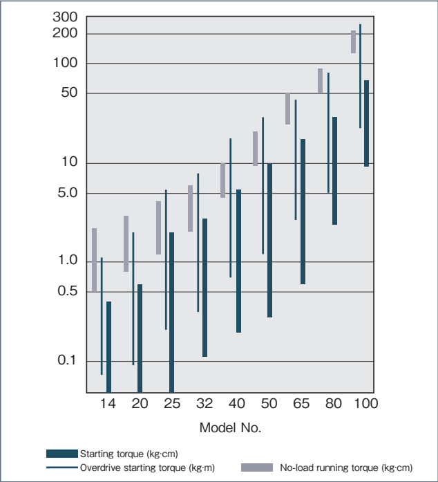
Running torque, starting torque, overdrive starting torque Graph 119-1
