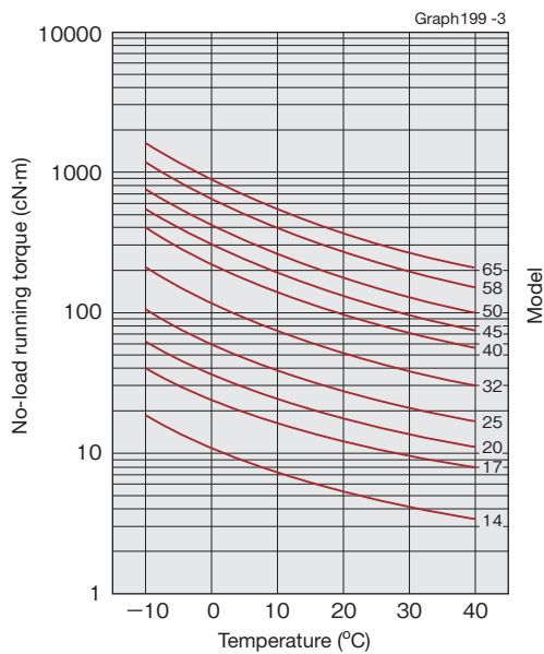
Input rotational speed: 2000r/min
