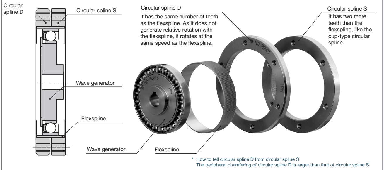
Structure of the FB series component type
