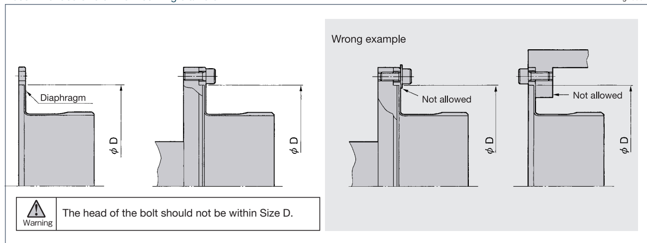
Recommended size of the mounting diameter
