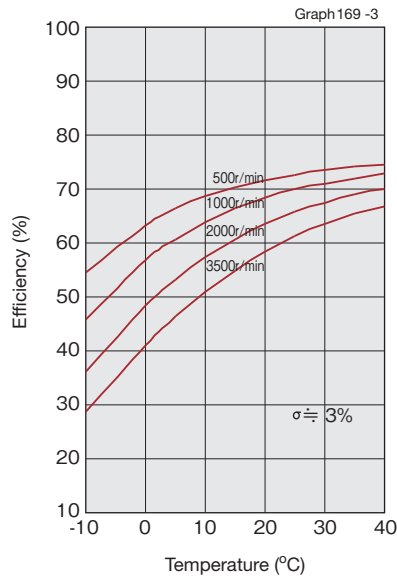
Model 17 to 40/ Reduction ratio 50
