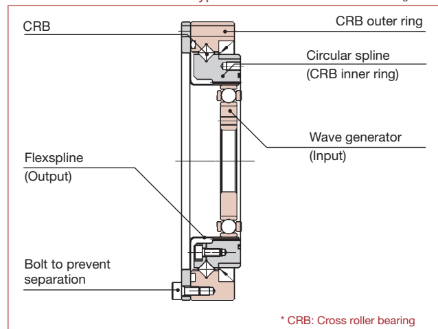
Structure of SHD series unit type
