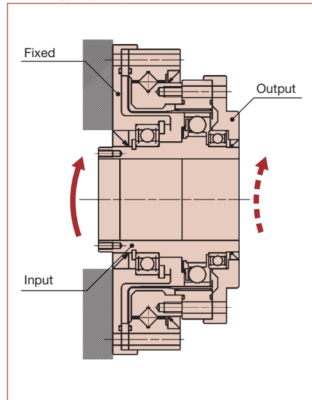
Hollow type (2UH)
