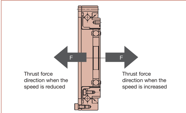
Thrust force direction of the wave generator
