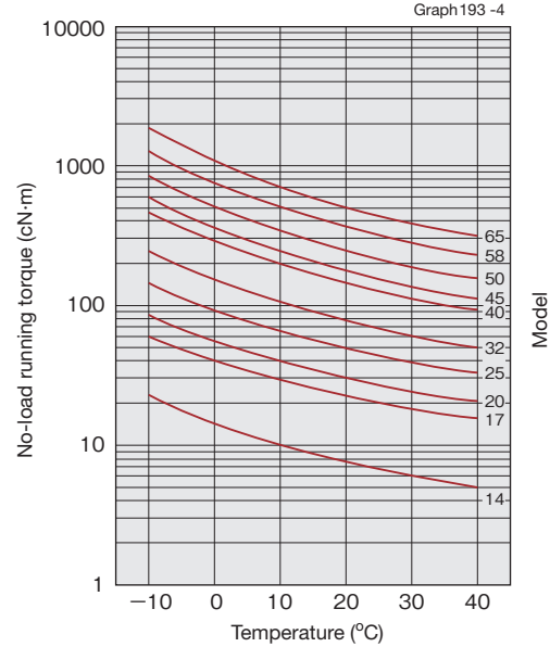
SHG/SHF-14 to 65 Reduction ratio: 100 Input rotational speed: 3500r/min
