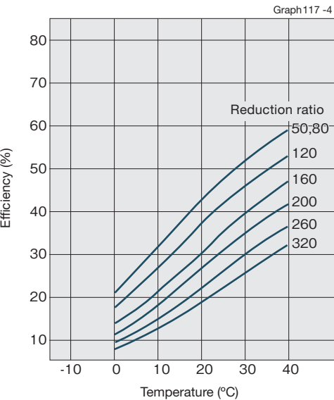
Input rotational speed: 3500r/min
