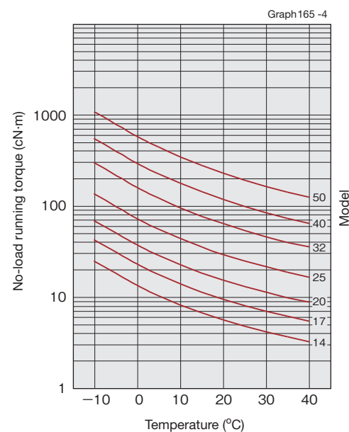
Input rotational speed: 3500r/min
