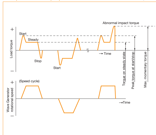
Example of load torque pattern
