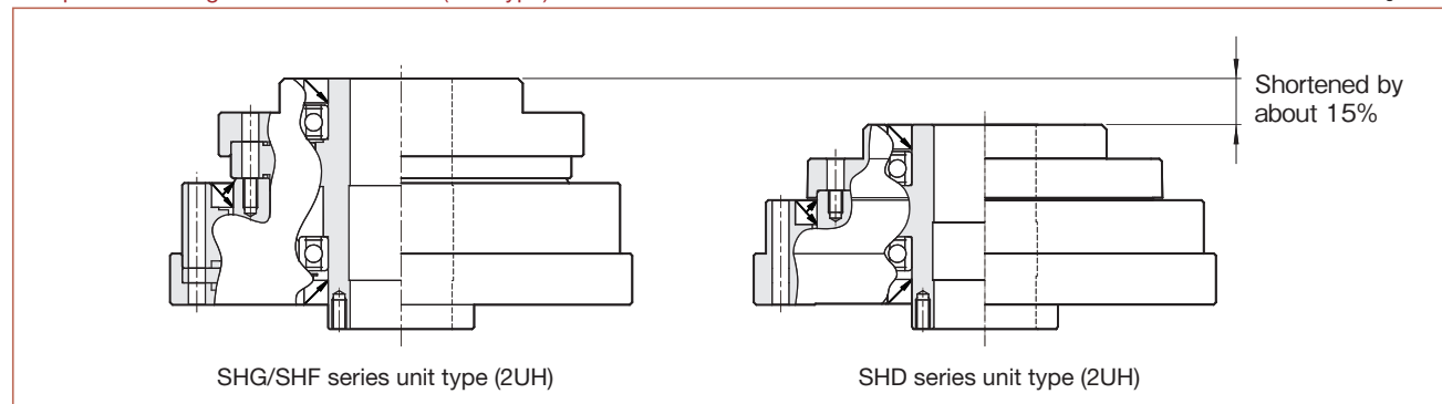
Comparison of lengths of shaft direction (Unit type)
