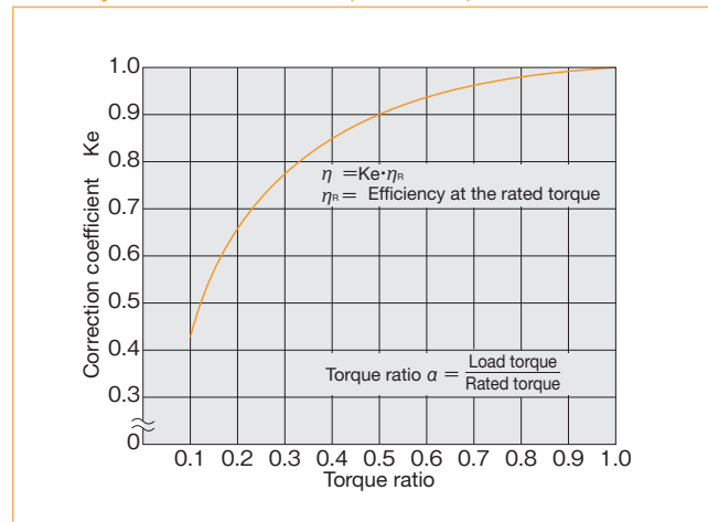
Efficiency correction coefficient (CSF series)
