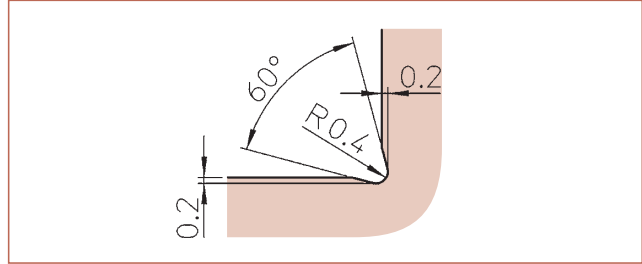
Recommended recessing size on the other side of installation
