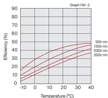
SHF-11 Reduction ratio 100
