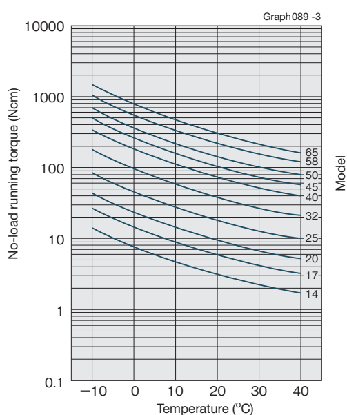
Input rotational speed: 2000r/min
