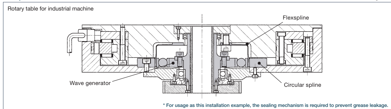
Example of CSD series installation
