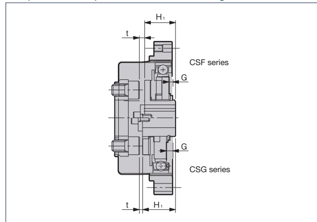
Comparison of shapes and sizes of the wave generator
