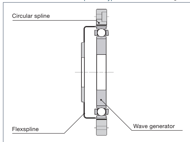
Structure of CSD series component type
