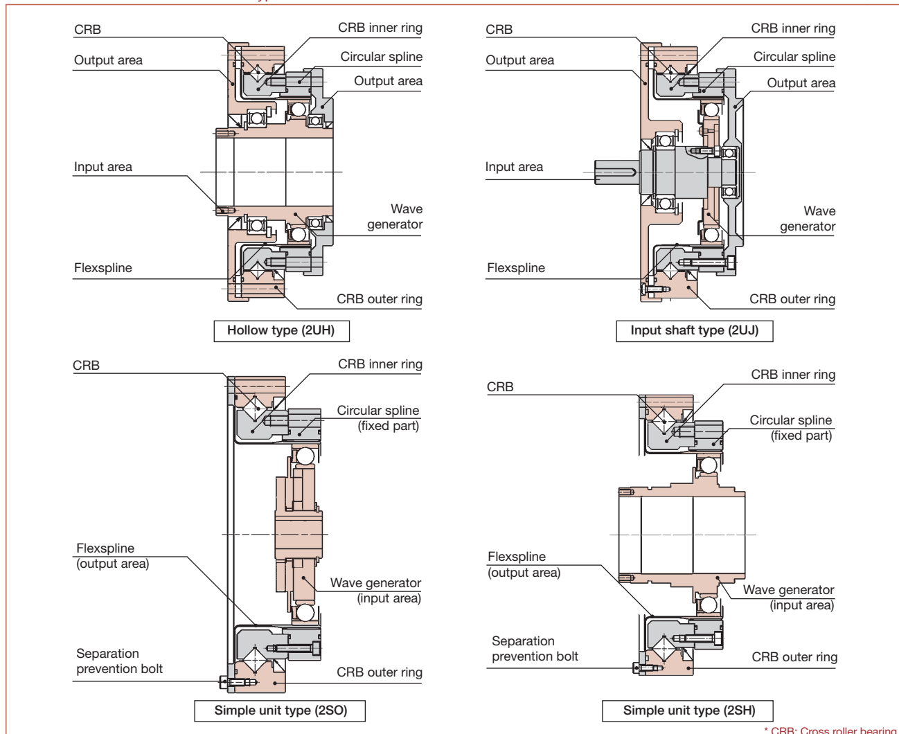
Structure of the SHG/SHF series unit type
