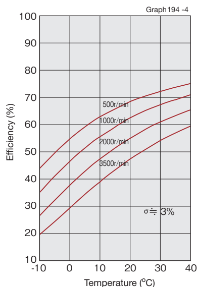
SHG/SHF-14 to 65 Reduction ratio 50, 80, 100, 120
