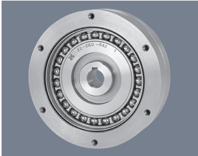
Structure of the FR series component type
