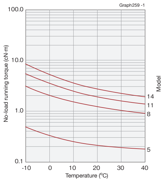
Input rotational speed: 2000r/min
