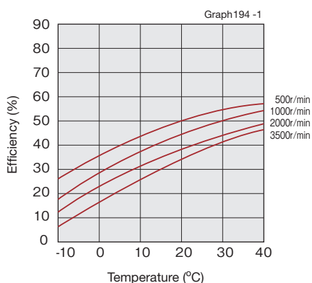
SHF-11 Reduction ratio 50
