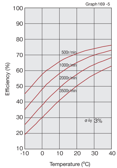
Model 20 to 40/ Reduction ratio 160
