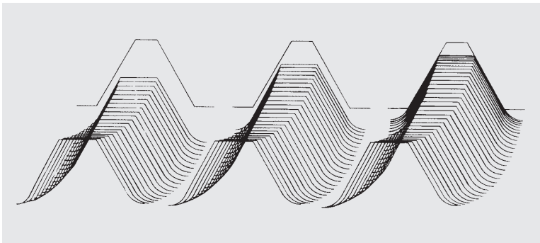
Conventional tooth profile
