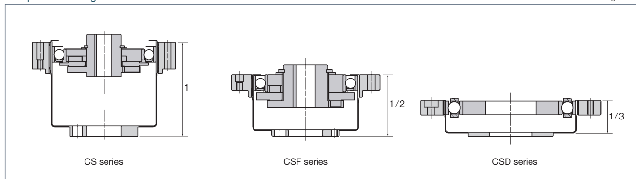
Comparison of lengths of shaft direction
