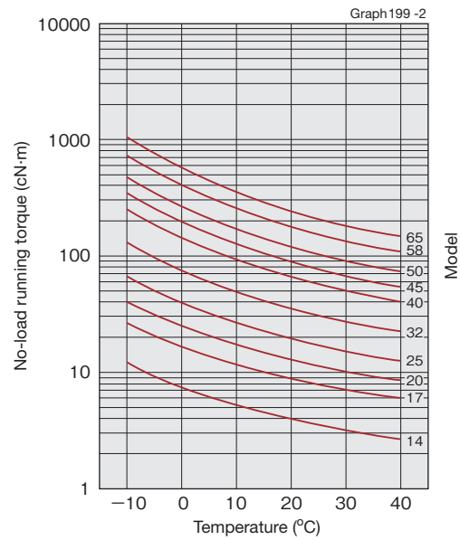
Input rotational speed: 1000r/min
