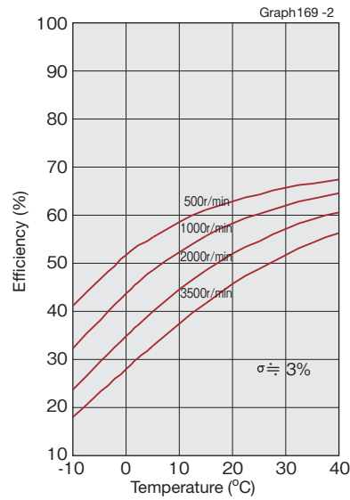
Model 14/ Reduction ratio 80, 100, 120
