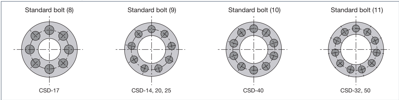
Numbers of holes and hole positions of bolts
