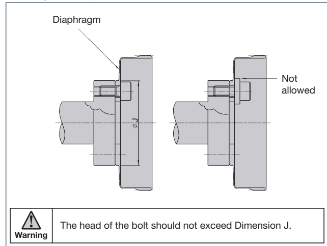
Installing the flexspline
