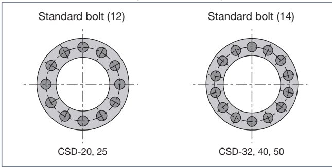
Numbers of holes and hole positions of BB specification
