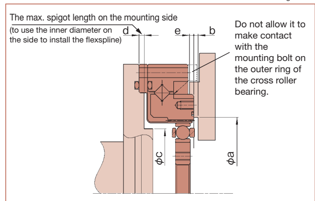
Recommended size for the inner wall of the case
