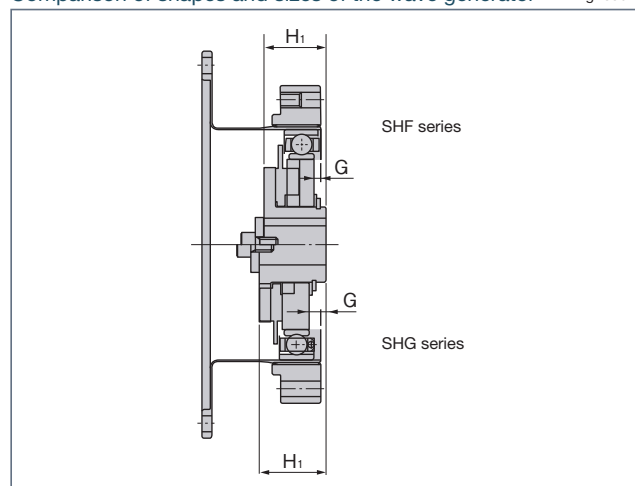
Comparison of shapes and sizes of the wave generator
