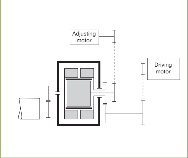
Using the Harmonic differential gear
