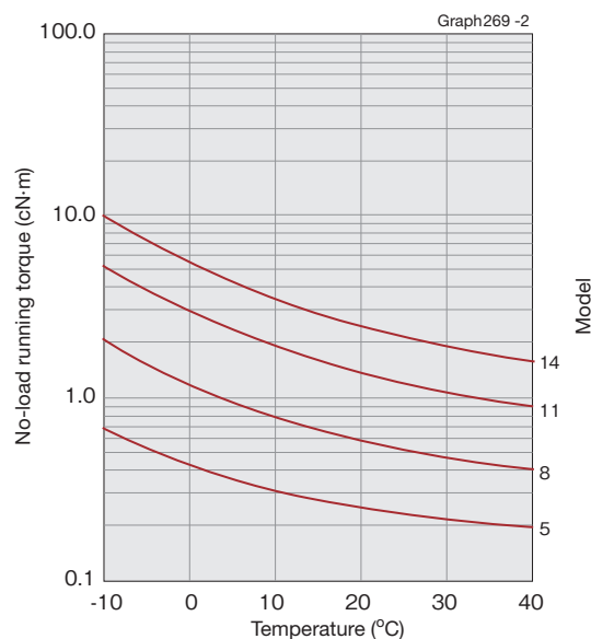
Input rotational speed: 1000r/min
