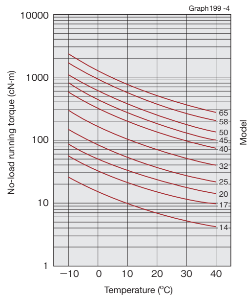
Input rotational speed: 3500r/min
