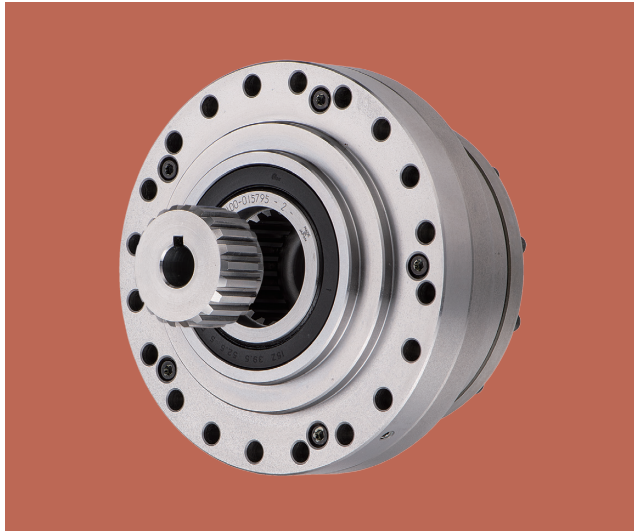
CSG Series Seal Structure Full Unit Type
