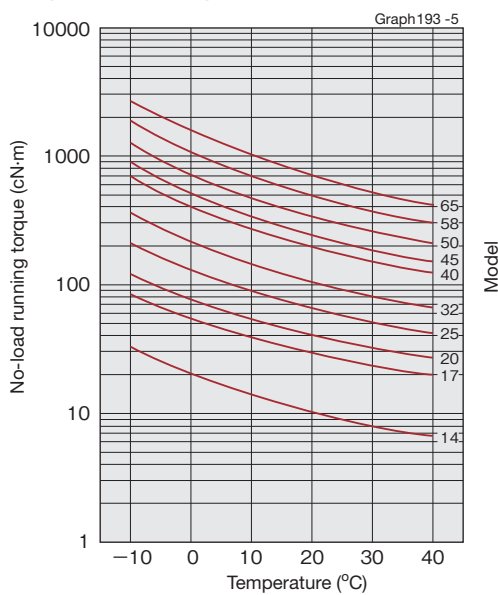
SHG/SHF-14 to 65 Reduction ratio: 100 Input rotational speed: 2000r/min
