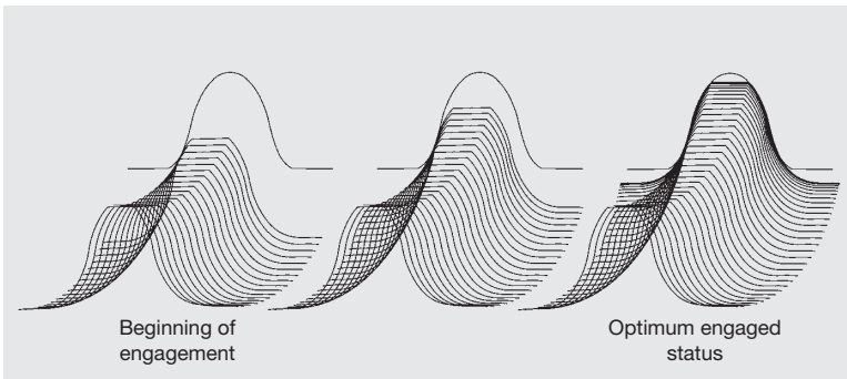
IH tooth profile
