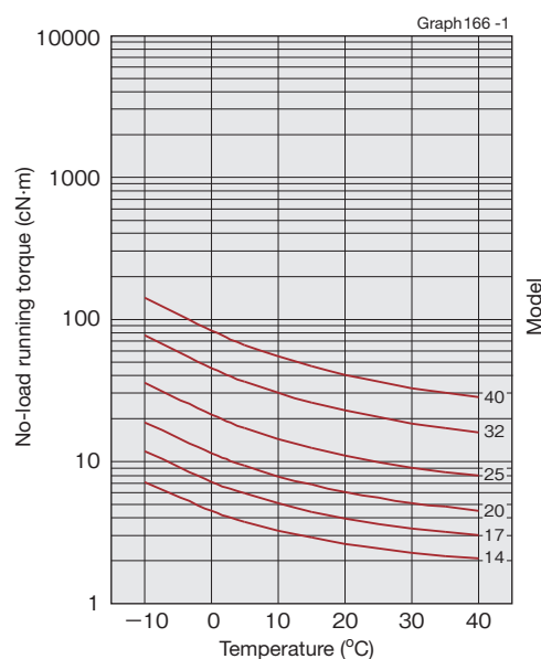
Input rotational speed: 500r/min
