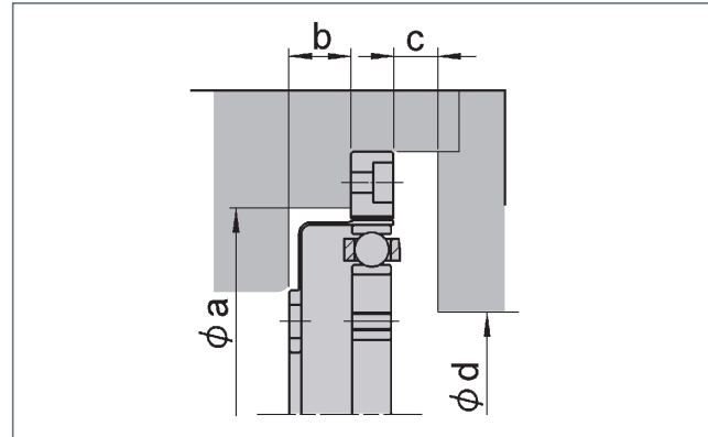
Recommended size for the inner wall of the case
