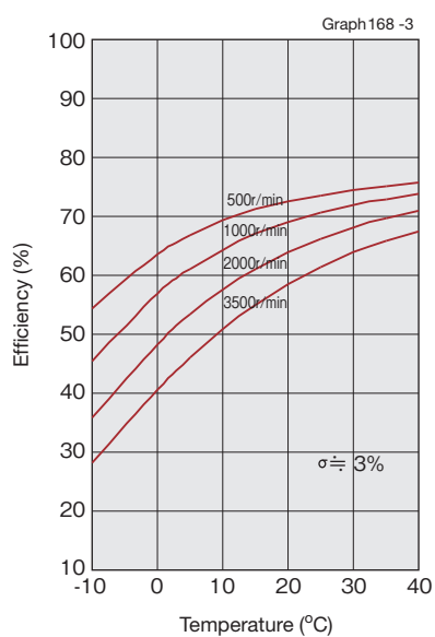
Model 17 to 50/ Reduction ratio 50
