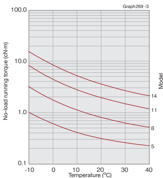
Input rotational speed: 2000r/min
