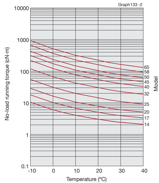
Input rotational speed: 3500r/min
