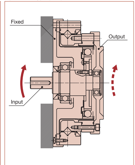
Input shaft type (2UJ)
