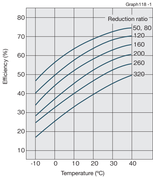
Input rotational speed: 500r/min
