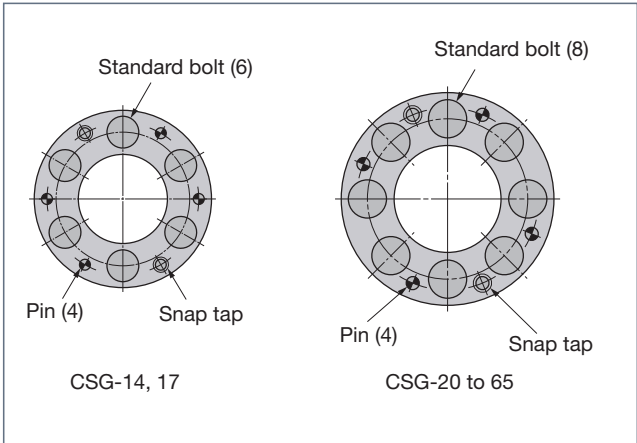
CSG series: Hole positions of bolts and pins
