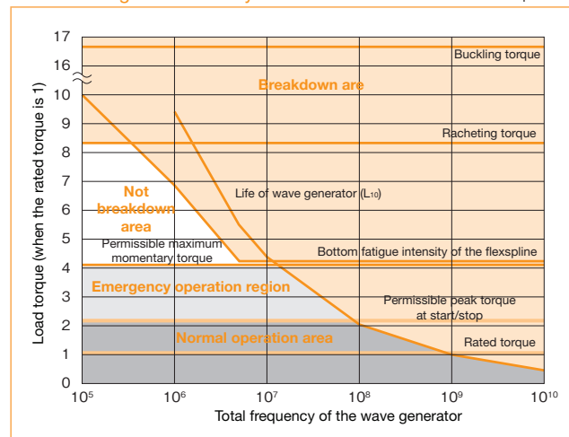
Relational diagram of intensity and life of HarmonicDrive®
