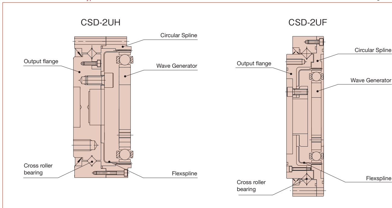
Structure of CSD series unit type
