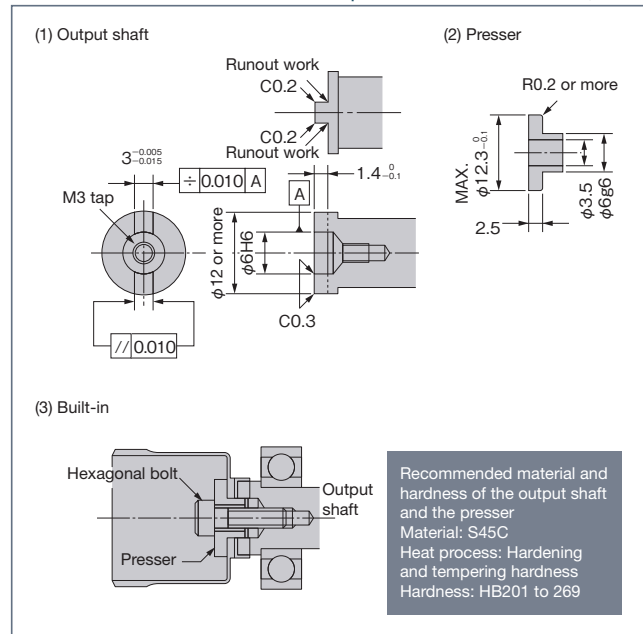
Installation of model number 8 flexspline
