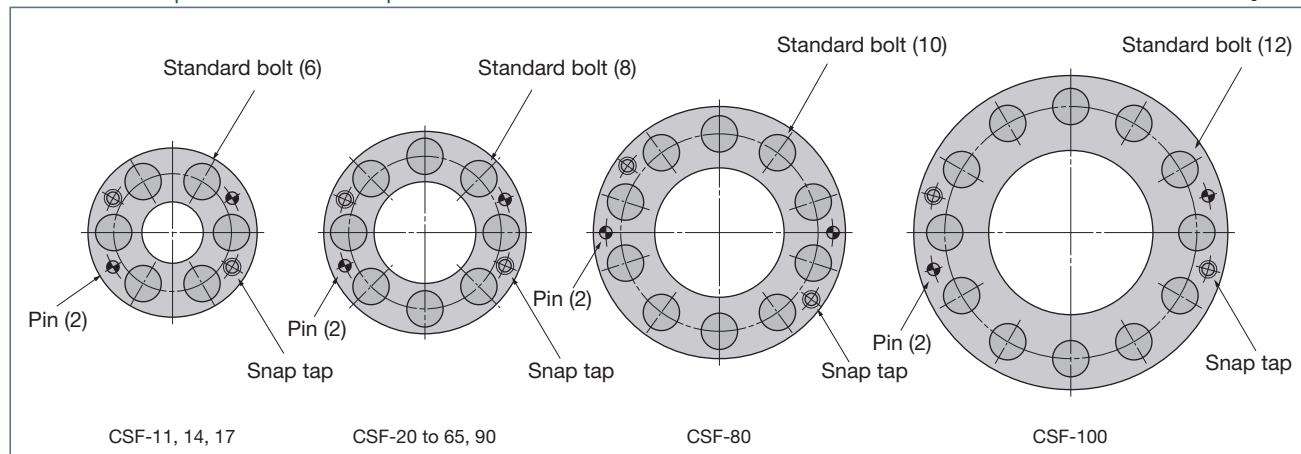
CSF series: Hole positions of bolts and pins
