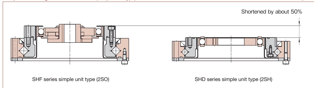
Comparison of lengths of shaft direction (Simple unit type)
