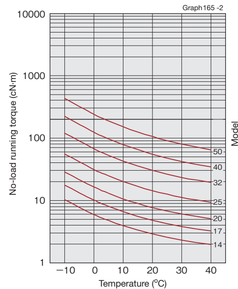
Input rotational speed: 1000r/min
