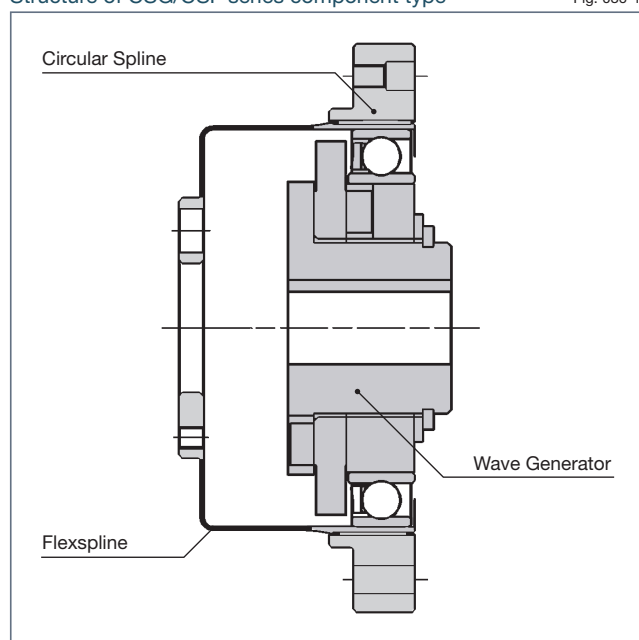
Structure of CSG/CSF series component type
