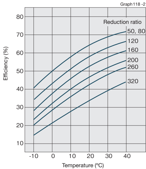
Input rotational speed: 1000r/min
