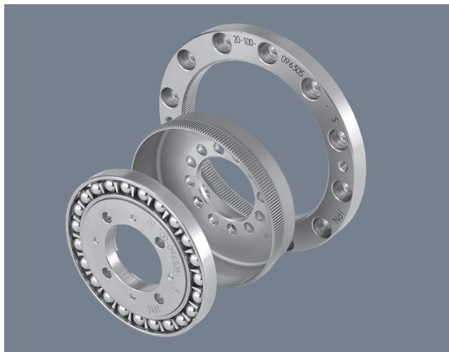
Structure of CSD series component type
