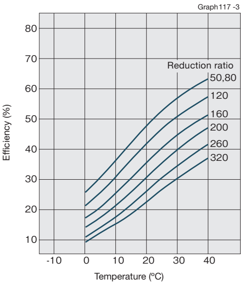
Input rotational speed: 2000r/min
