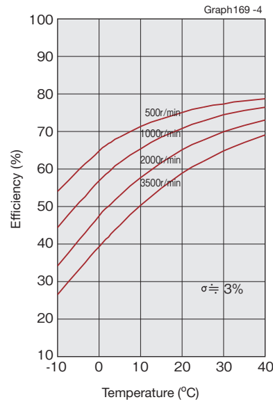
Model 17 to 40/ Reduction ratio 80, 100, 120
