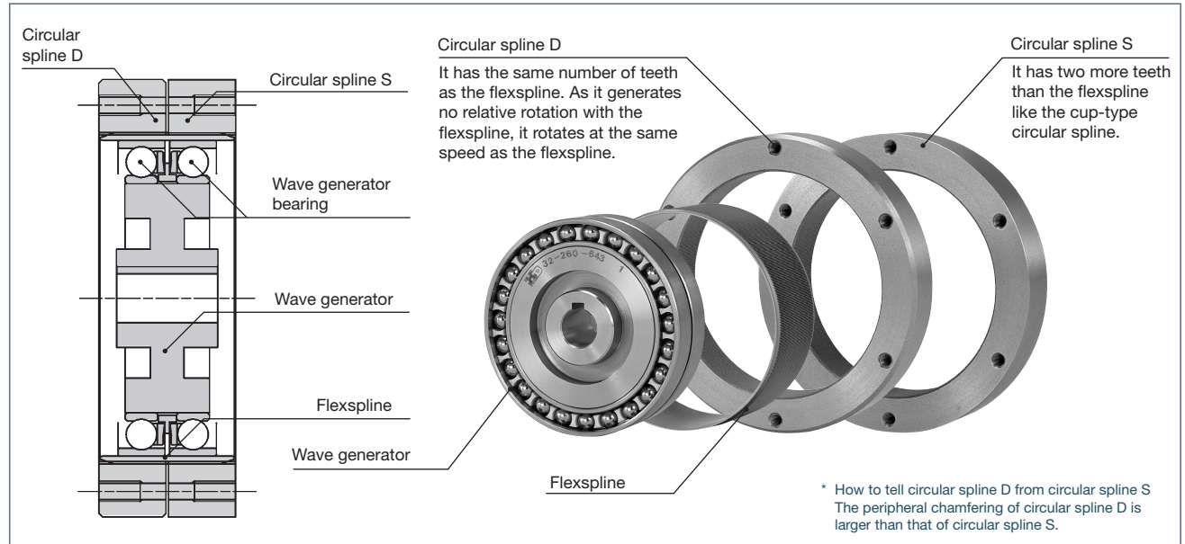
Structure of the FR series component type
